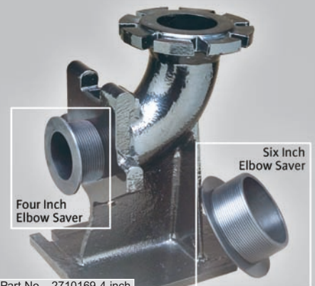
Part No. 2710169-4 inch Part No. 2710080-6 inch
